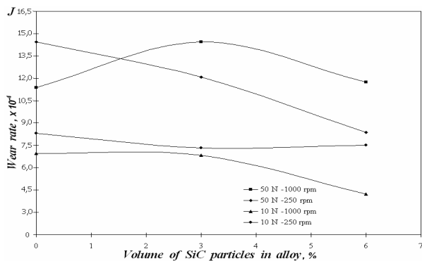
Figure 7. Dependence of wear rate on the volume of the powder filler
