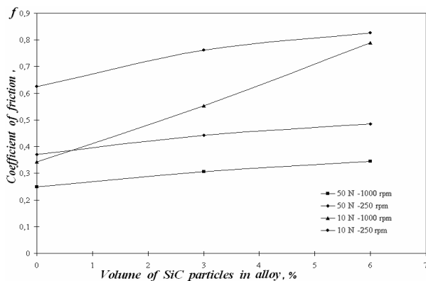
Figure 4. Friction coefficient dependence on the volume of powder filler
