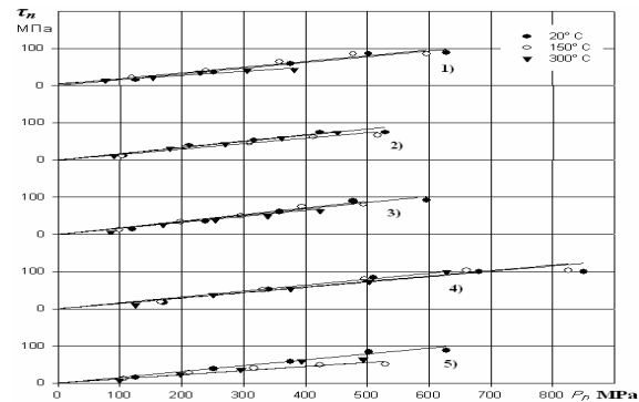
Figure 5 Dependence of adhesive shear bonds strength on normal pressure on the contact: 1) - AZ91D - SKD11; 2) - AZ91D + SiC ( S = 5 mcm; V = 3\% ) - SKD11; 3) - AZ91D + SiC ( S = 11 mcm; V = 3\% ) - SKD11; 4) - AZ91D + SiC ( S = 11 mcm; V = 6\% ) - SKD11; 5) - AZ91D + SiC ( S = 15 mcm; V = 3\% ) - SKD11
