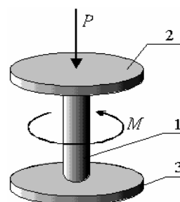
Figure 2. Test pattern for determining the molecular component of the friction coefficient: 1 – indenter; 2 – test specimens
