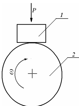
Figure 1. Test pattern: 1 – test specimen; 2 – revolving steel disc
