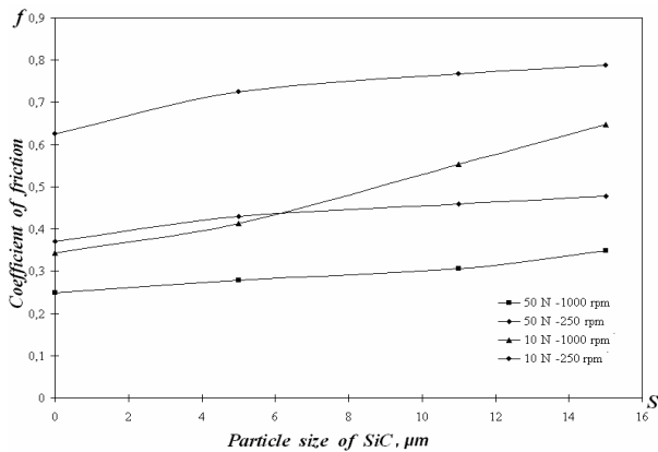
Figure 3. Friction coefficient dependence on particle size of silicone carbide
