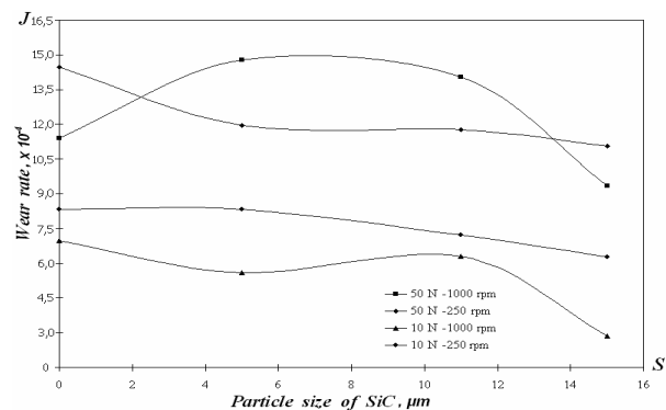
Figure 6. Dependence of wear rate on the particles size of SiC
